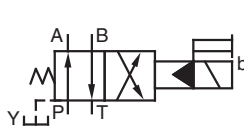
Standard Mtg. of Solenoid
