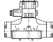
Reverse Mtg. of Solenoid ("L")
