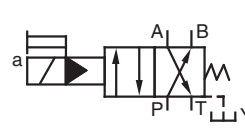
Reverse Mtg. of Solenoid ("L")
